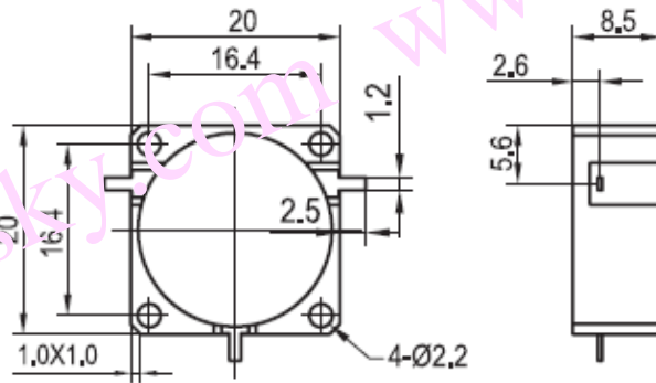
DC080SA 安装图
