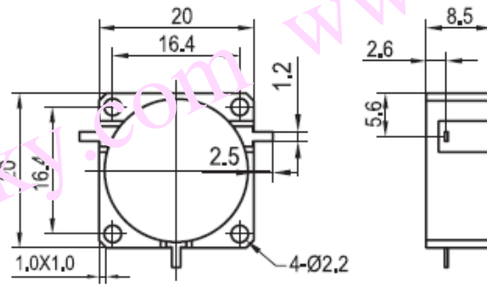
DC080SA 安装图
